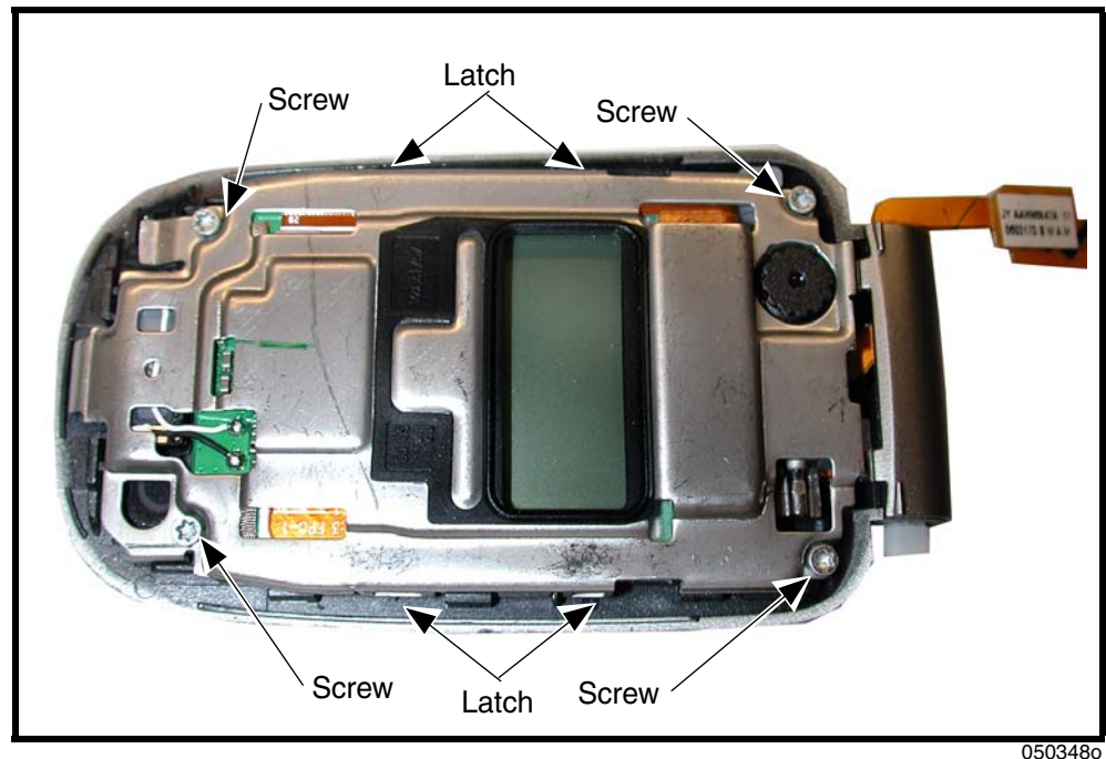
Figure 15. Removing the Flip Assembly Screws and Latches
