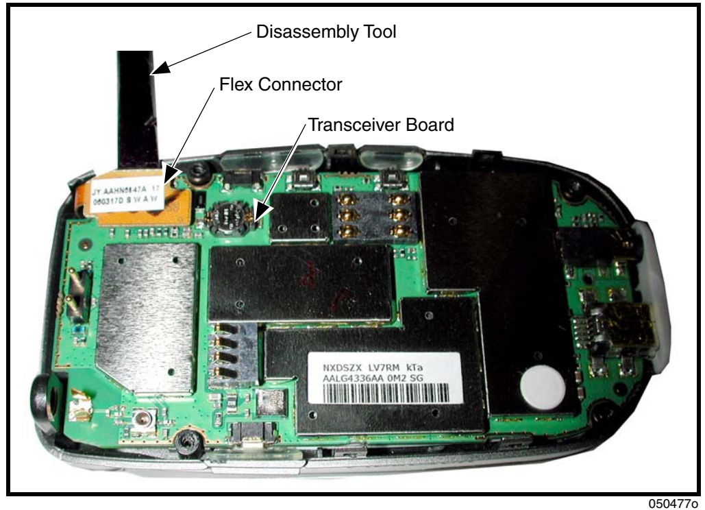
Figure 8. Disconnecting the Flex from the Transceiver Board
