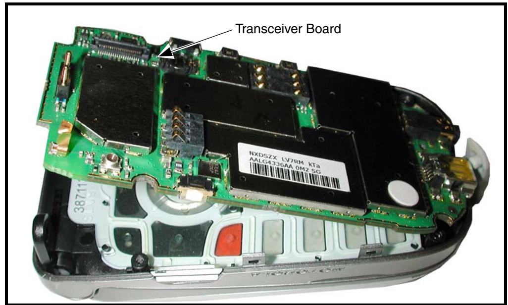
Figure 9. Removing the transceiver PC board assembly
