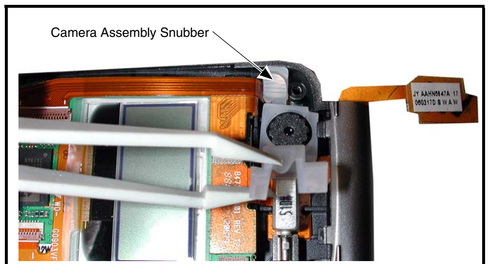
Figure 16. Camera Assembly Snubber Removal
