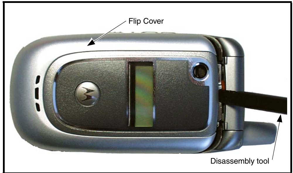
Figure 14. Removing the Flip Cover
