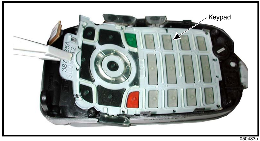
Figure 10. Removing the Keypad, Volume/Smart, and Voice Buttons
