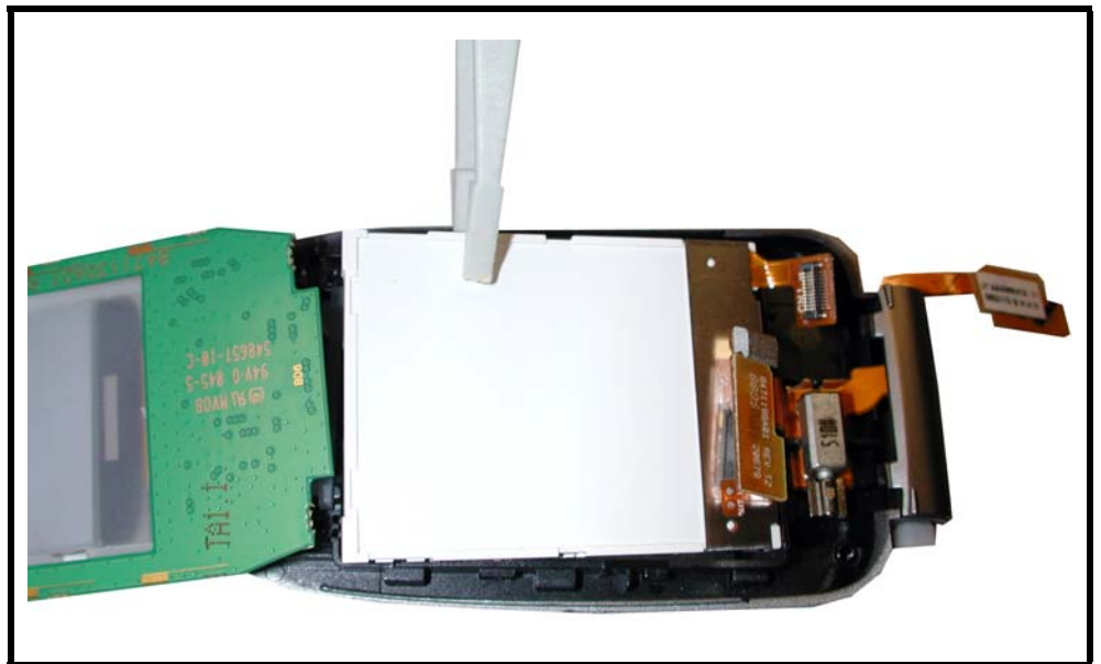
Figure 21. Display Module Removal
