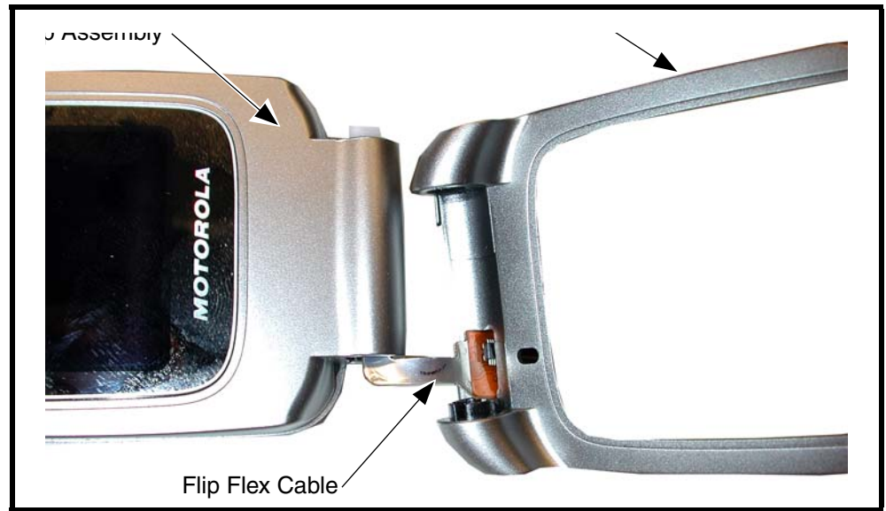
Figure 13. Removing the Flip Assembly
