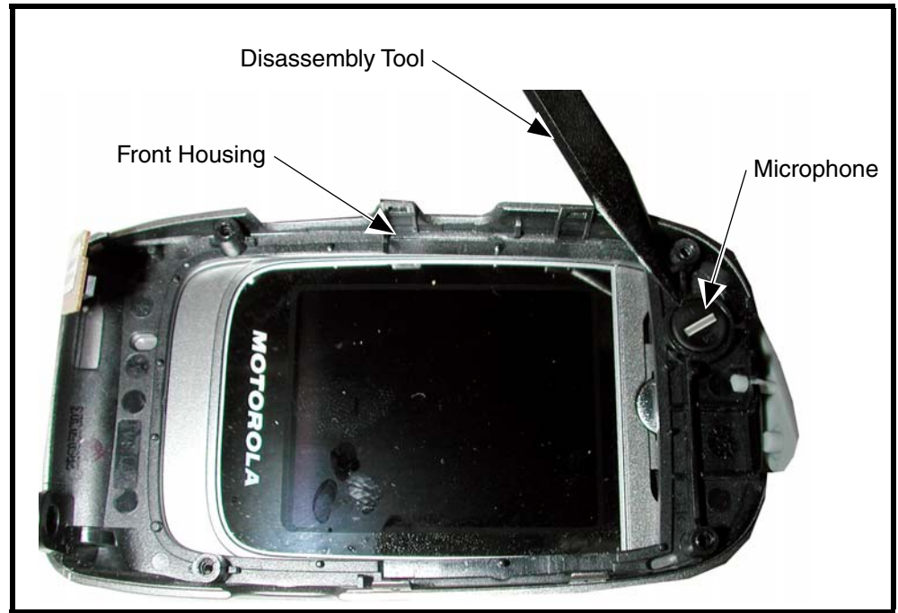
Figure 11. Removing the Microphone
