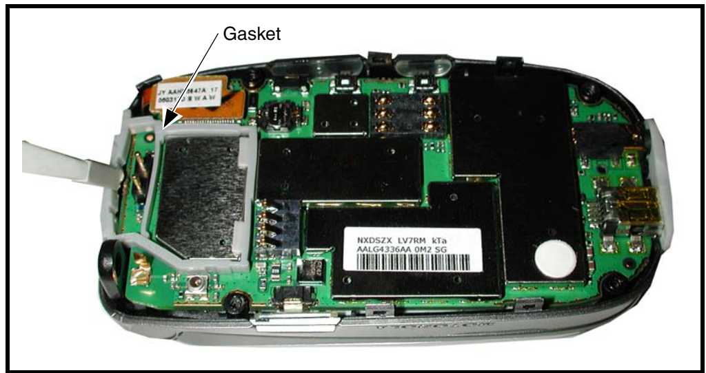
Figure 7. Removing the Gasket From the Transceiver Board
