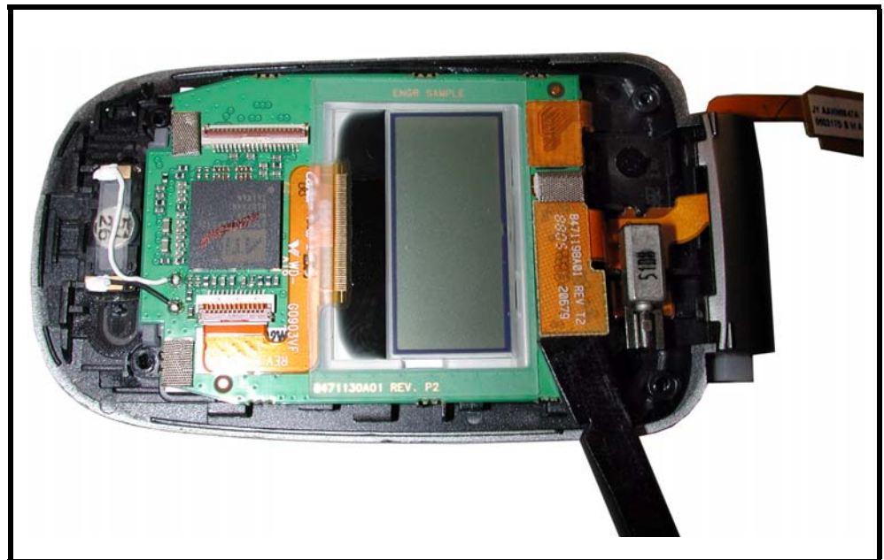
Figure 19. Display Flex Connector Removal
