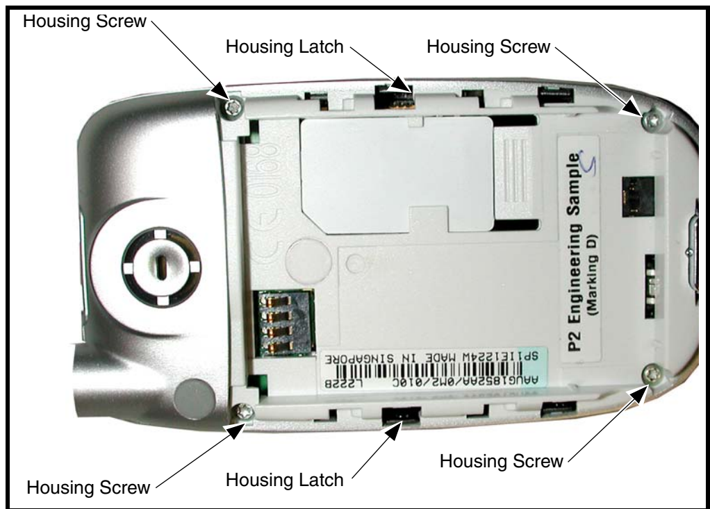
Figure 5. Removing the Rear Housing Screws
